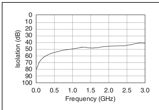
Figure 4. Typical Isolation
