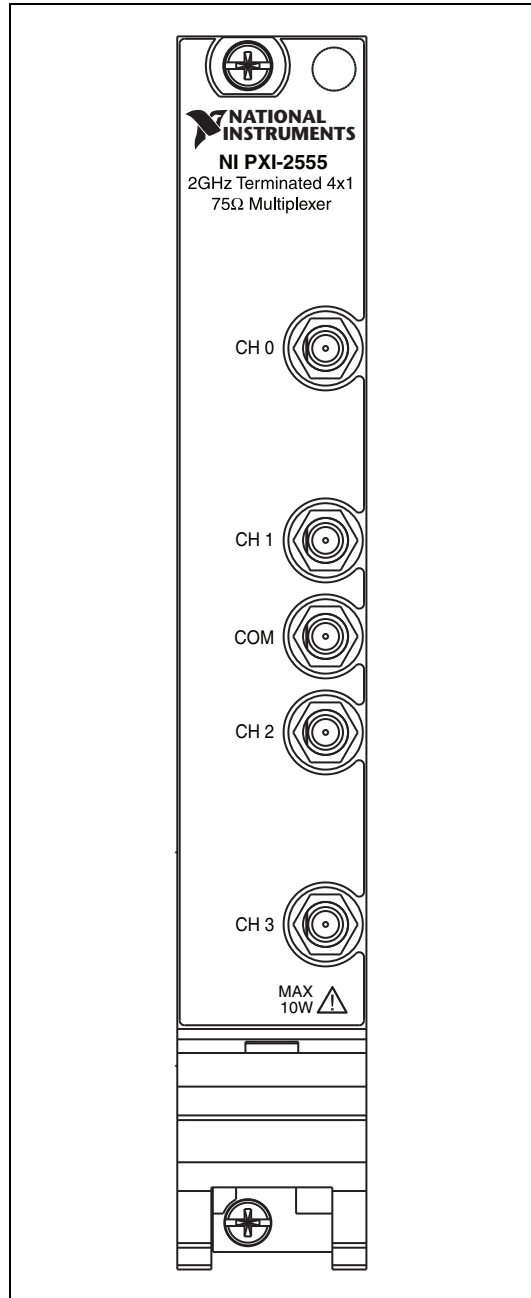
Figure 7. NI PXI-2555 Front Panel Connector
