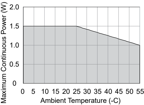
Figure 5. Termination Derating
