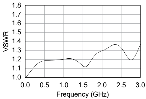
Figure 3. Typical Termination VSWR
