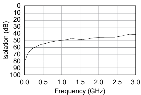
Figure 4. Typical Isolation
