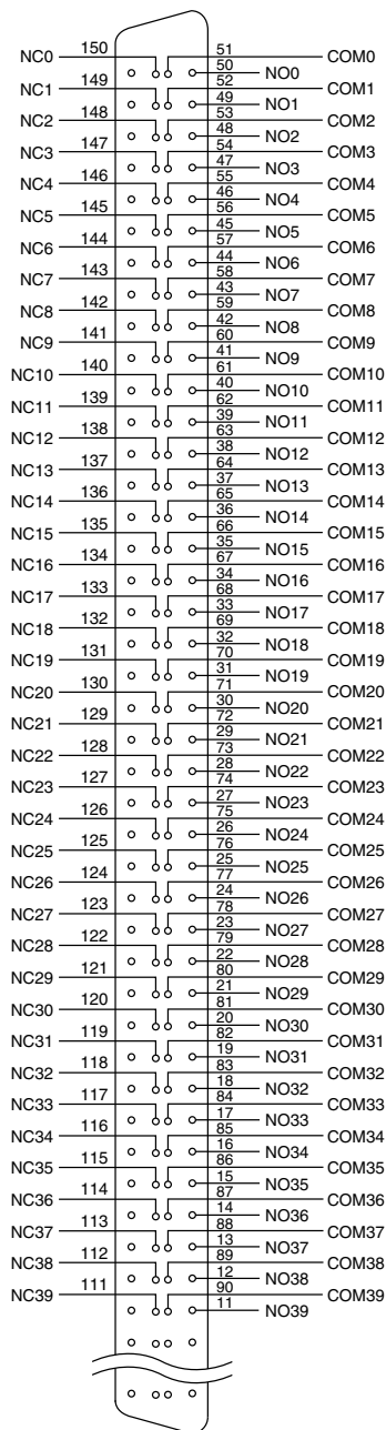
Figure 2. PXI-2570 Connector Pinout
