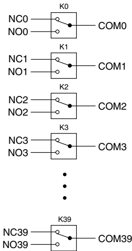
Figure 1. PXI-2570 Power-on State
