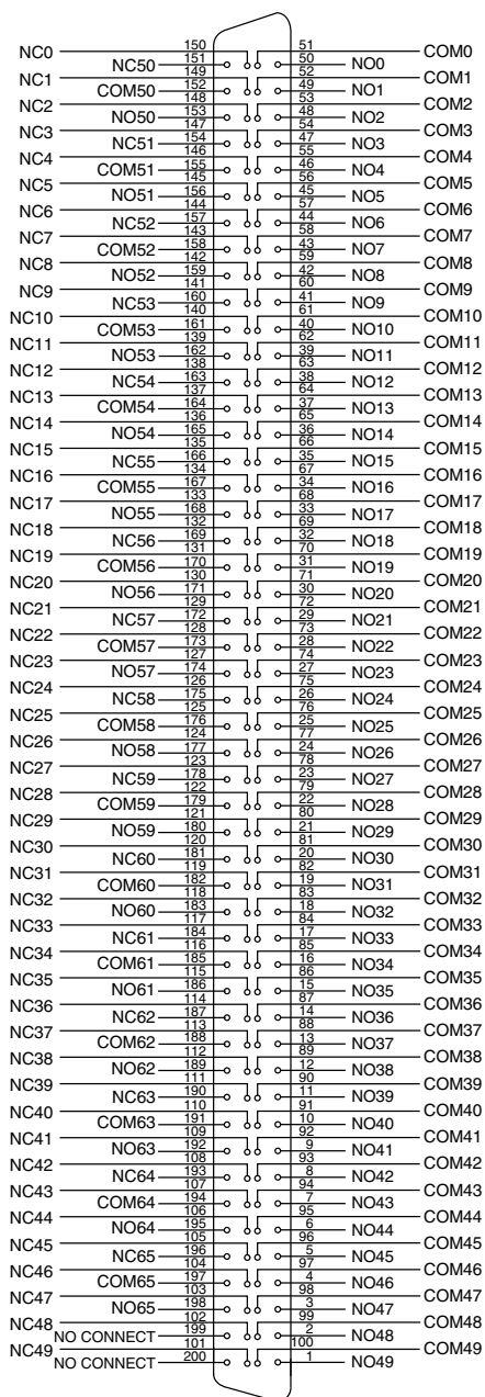
Figure 2. PXI-2571 Connector Pinout
