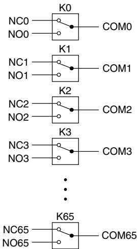
Figure 1. PXI-2571 Power-on State
