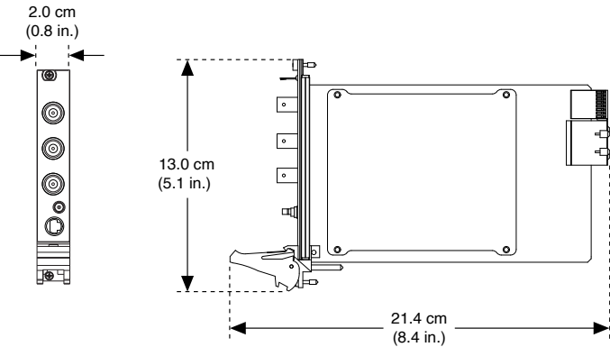
Figure 3. PXIe-5114
