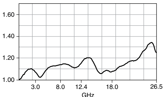
Figure 2. VSWR, Typical
