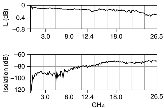
Figure 1. Insertion Loss and Isolation, Typical
