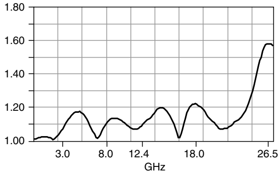
Figure 2. VSWR, Typical
