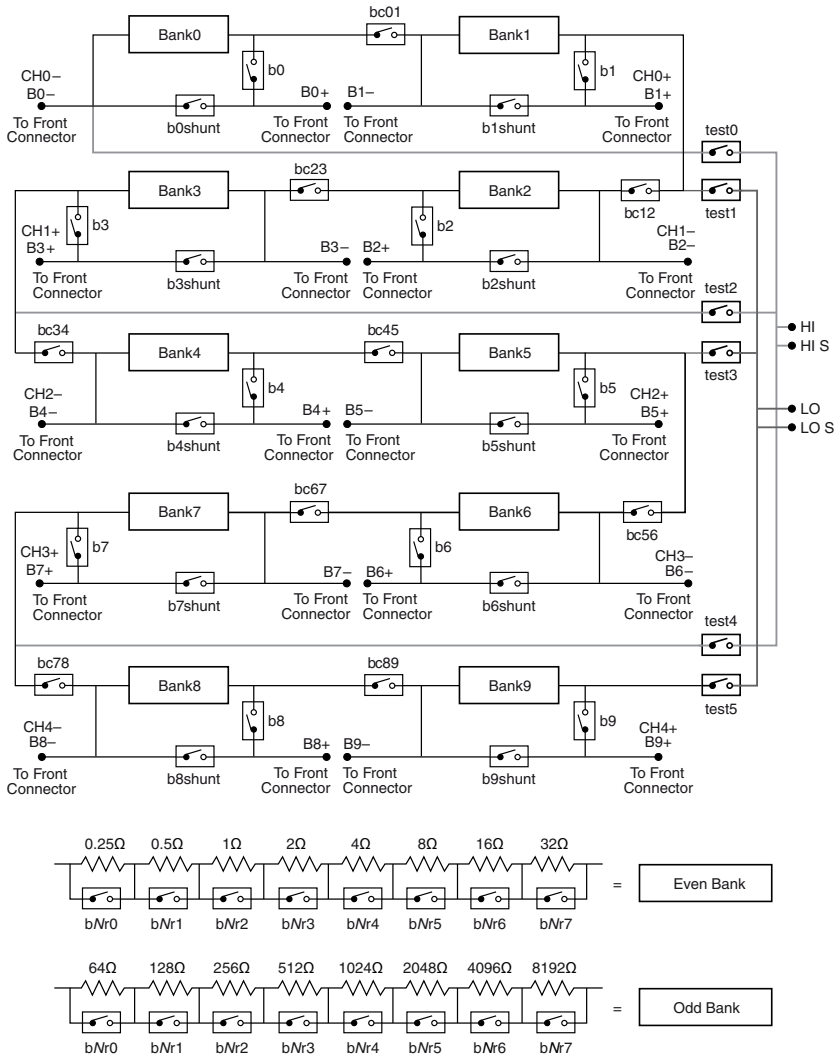
Figure 6. NI 2722 Power-on State
