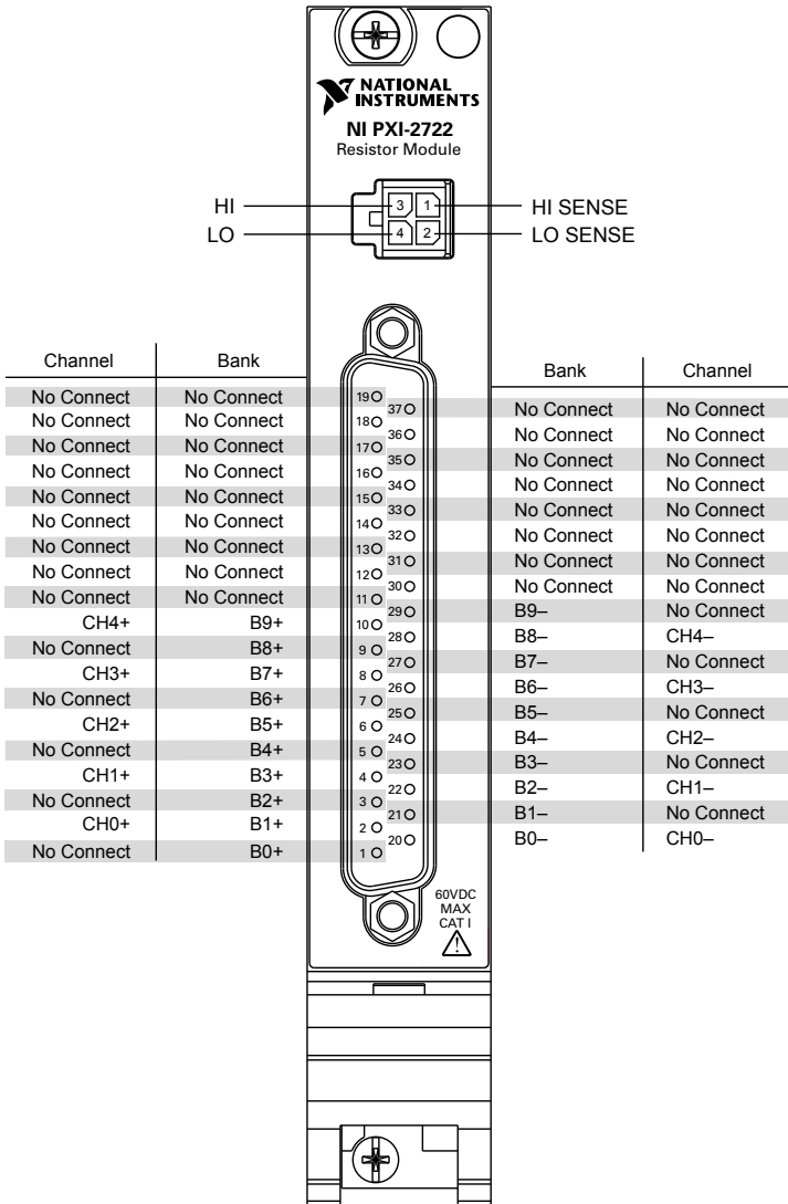
Figure 5. NI 2722 Connector Pinout
