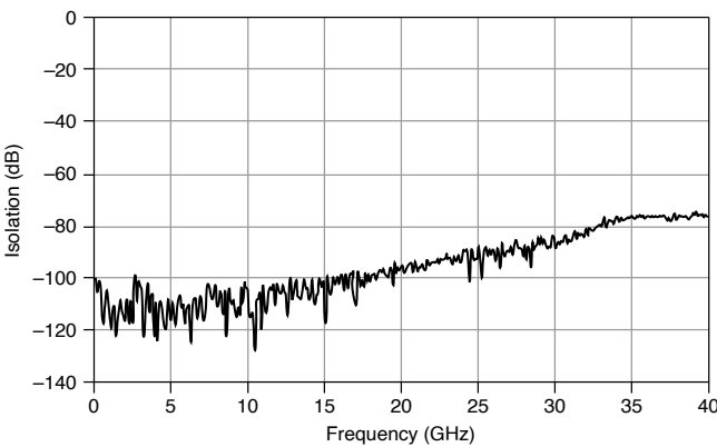
Figure 2. Typical Isolation
