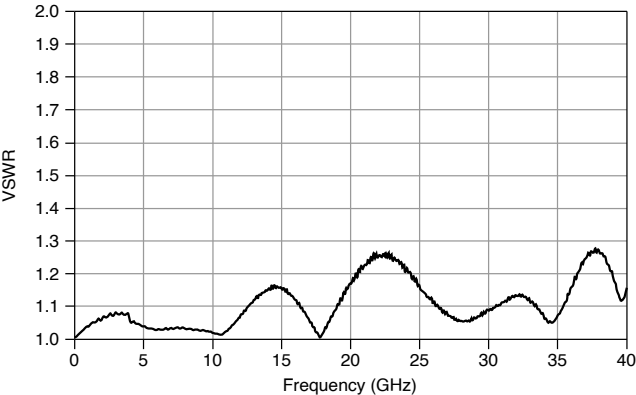
Figure 3. Typical VSWR
