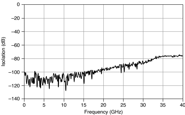
Figure 2. Typical Isolation
