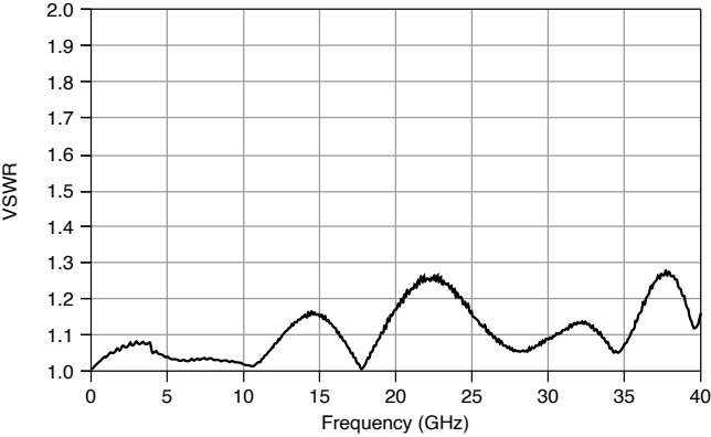
Figure 3. Typical VSWR
