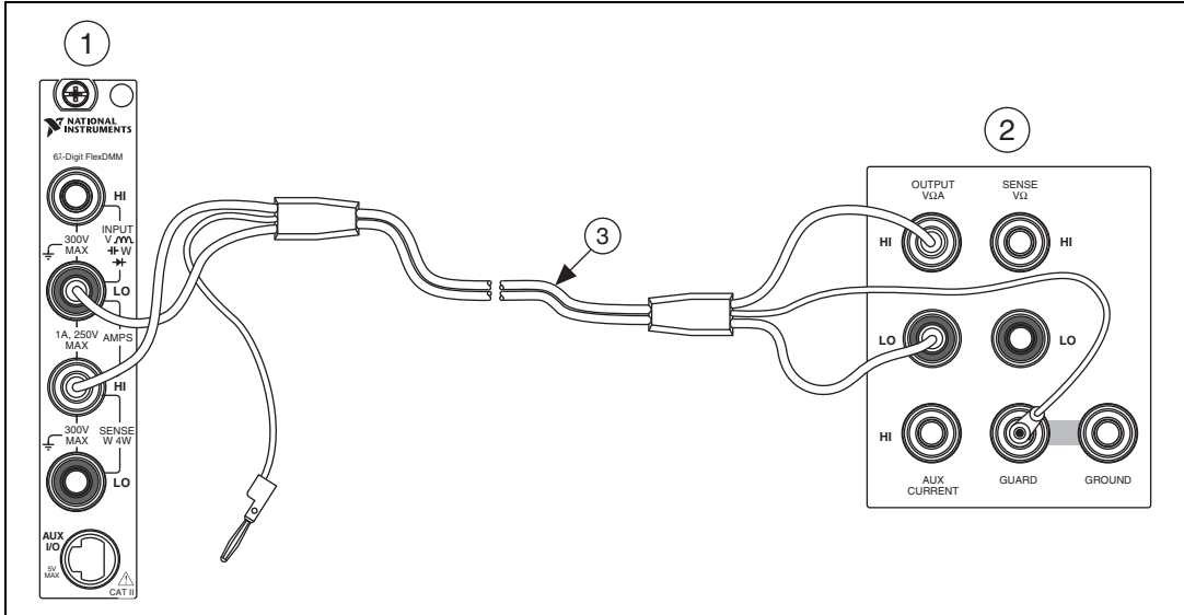
1 NI 4070/4072 2 Fluke 5700A/5720A Calibrator 3 Fluke 5440 Cable
