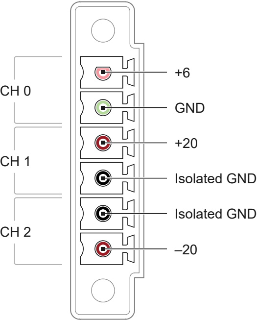
Figure 4. PXI-4110 Output Connector Pinout
