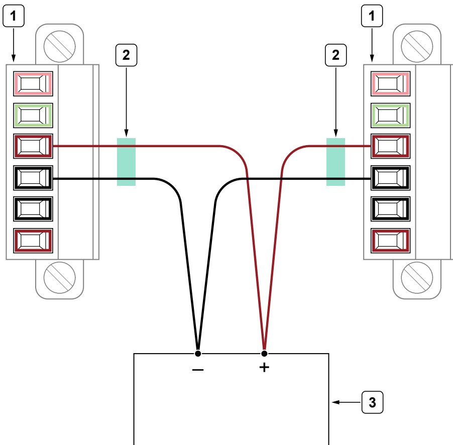
Figure 10. Parallel Connection Diagram
