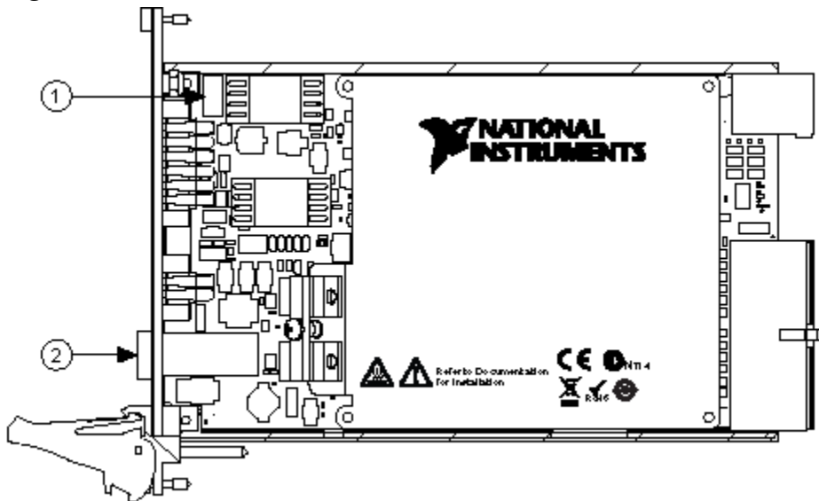
Figure 4. Fuse Locations
