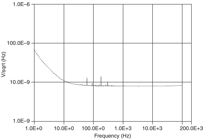
Figure 5. AI Spectral Noise Density (30 dB Gain)
