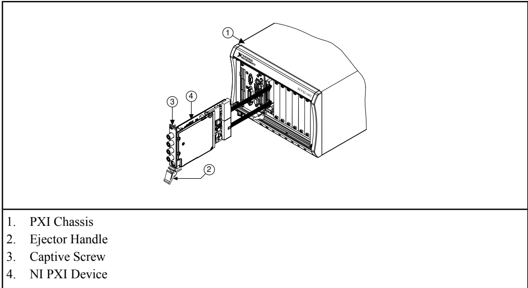
Figure 1. PXI Installation
