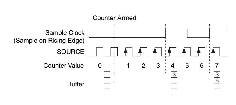
Figure 7-4. Buffered (Sample Clock) Edge Counting
