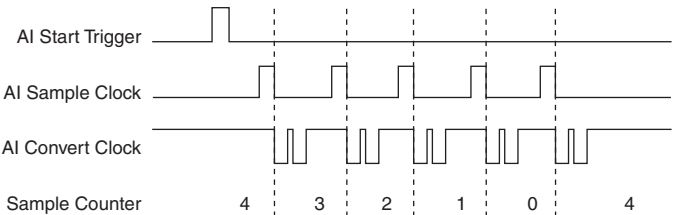
Figure 4-14. Posttriggered Data Acquisition Example
