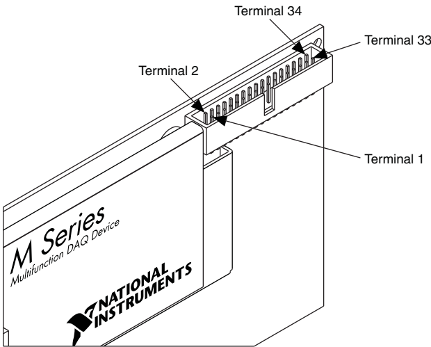
Figure 9-2. M Series PCI/PCI Express Device RTSI Pinout
