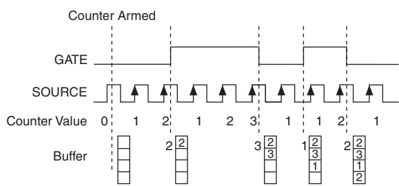
Figure 7-9. Buffered Semi-Period Measurement
