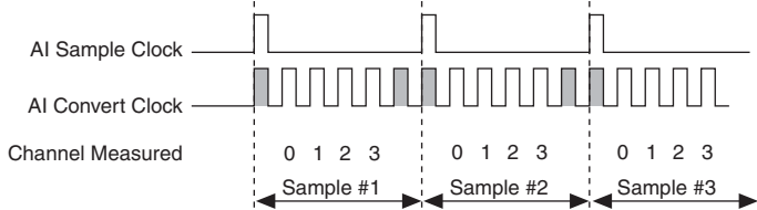
Figure 4-20. AI Sample Clock and AI Convert Clock Improperly Matched; Leads to Aperiodic Sampling
