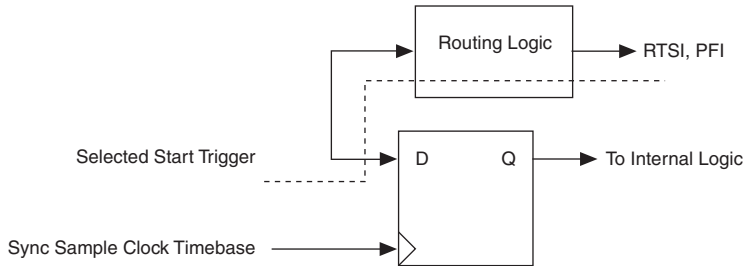
Figure B-32. Start Trigger Output Delay Timing Diagram
