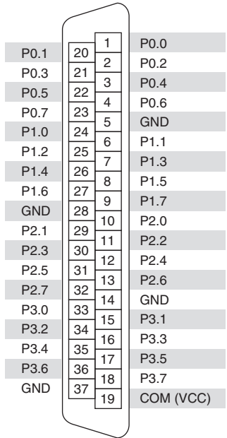
Figure 3-13. NI 6517 Pin Assignments
