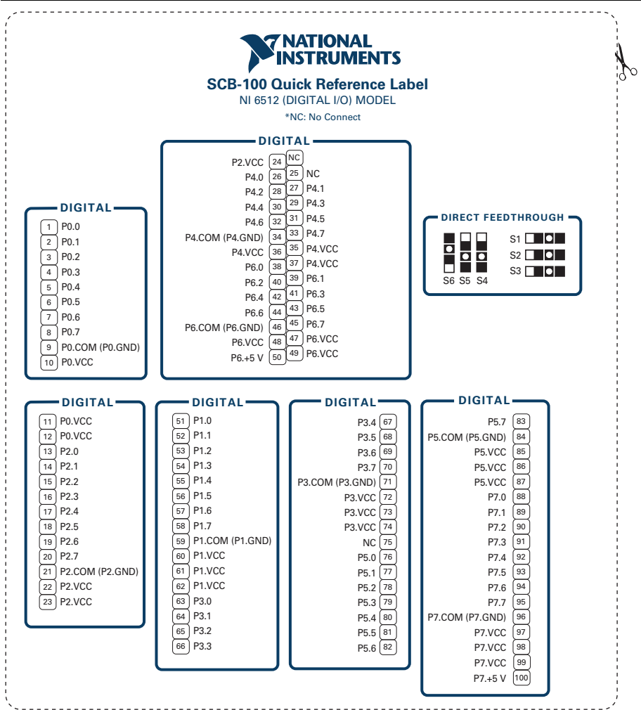
Figure 4. NI 6512
