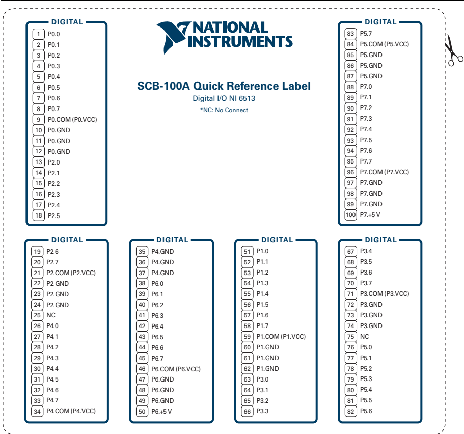
Figure 5. NI 6513
