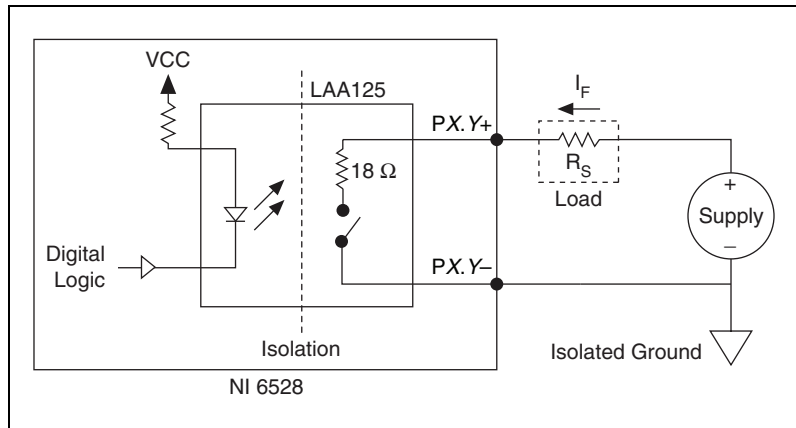
Figure 6. Sinking Current Connection Example
