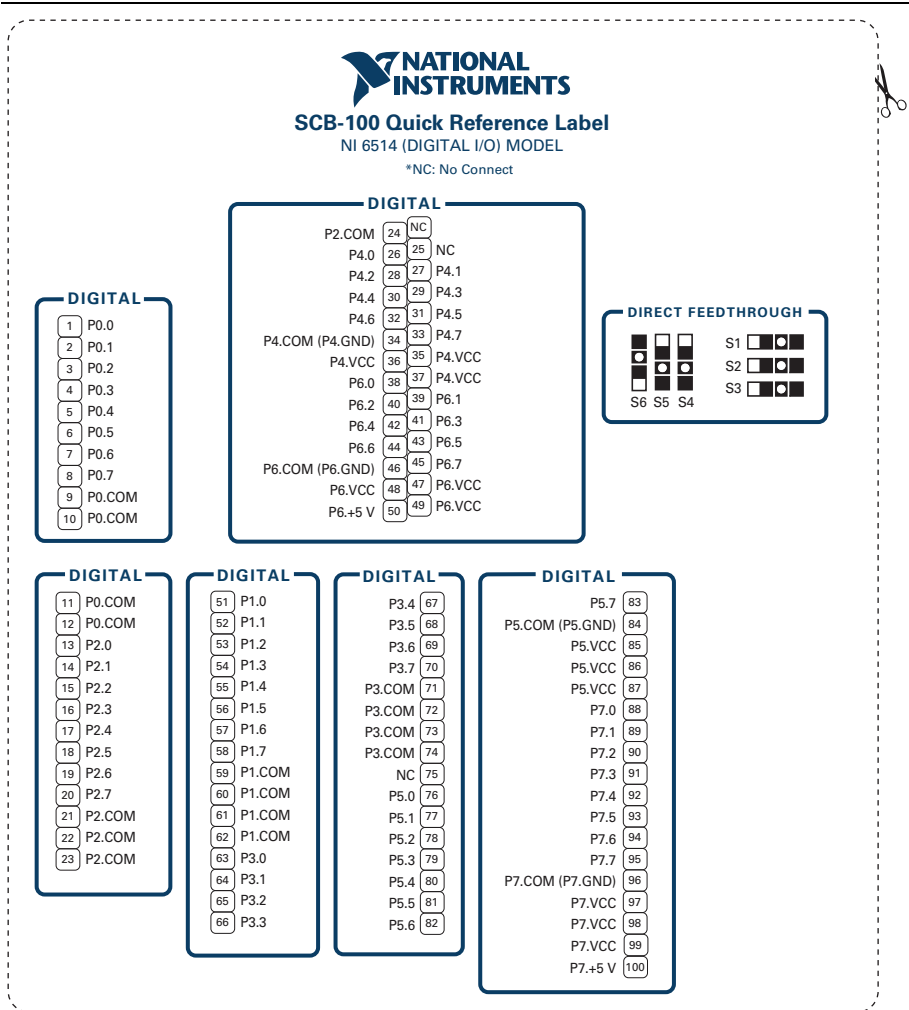
Figure 6. NI 6514
