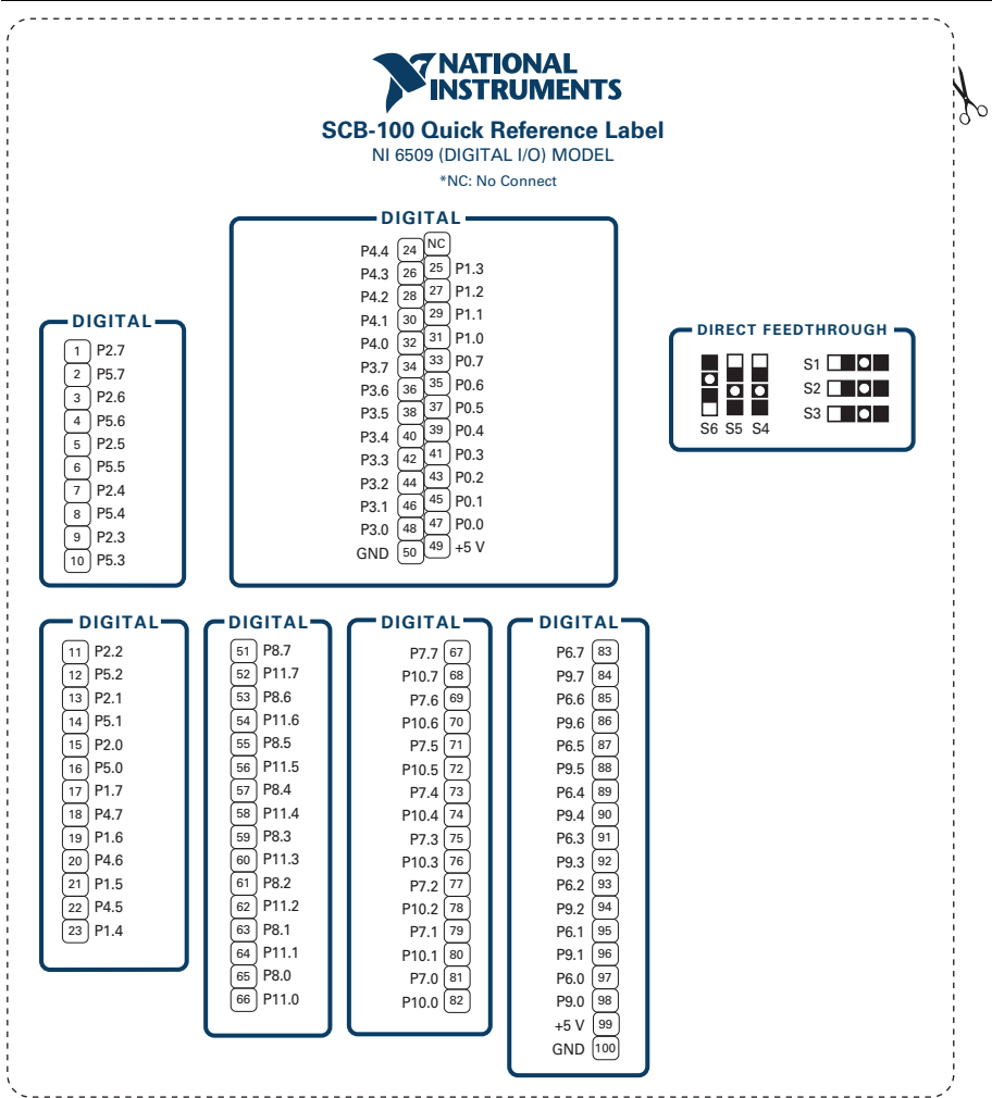
Figure 2. NI 6509
