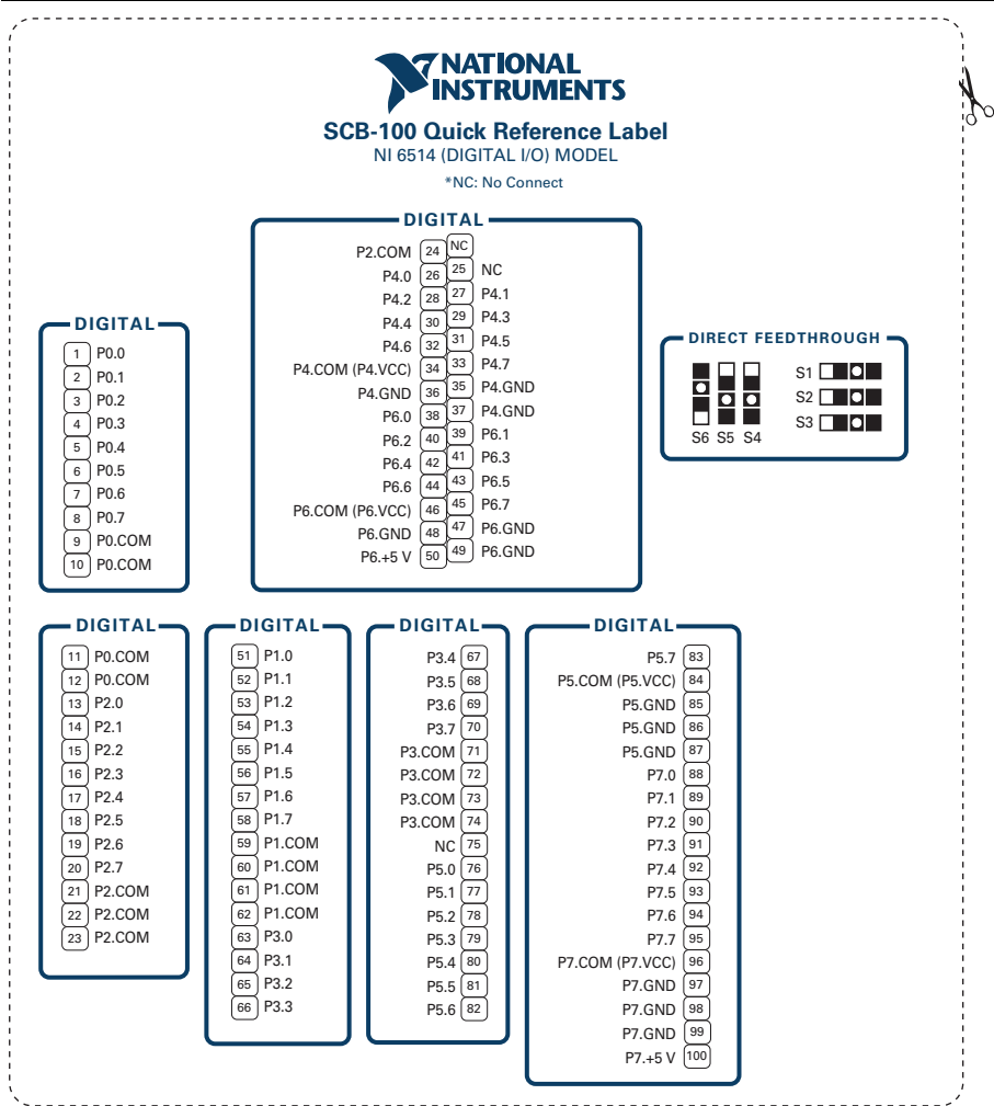
Figure 7. NI 6515
