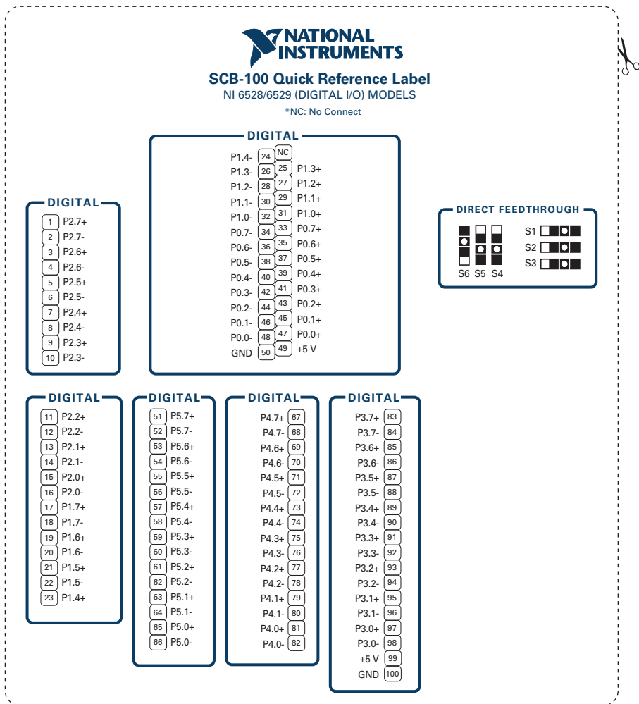
Figure 8. NI 6528/6529
