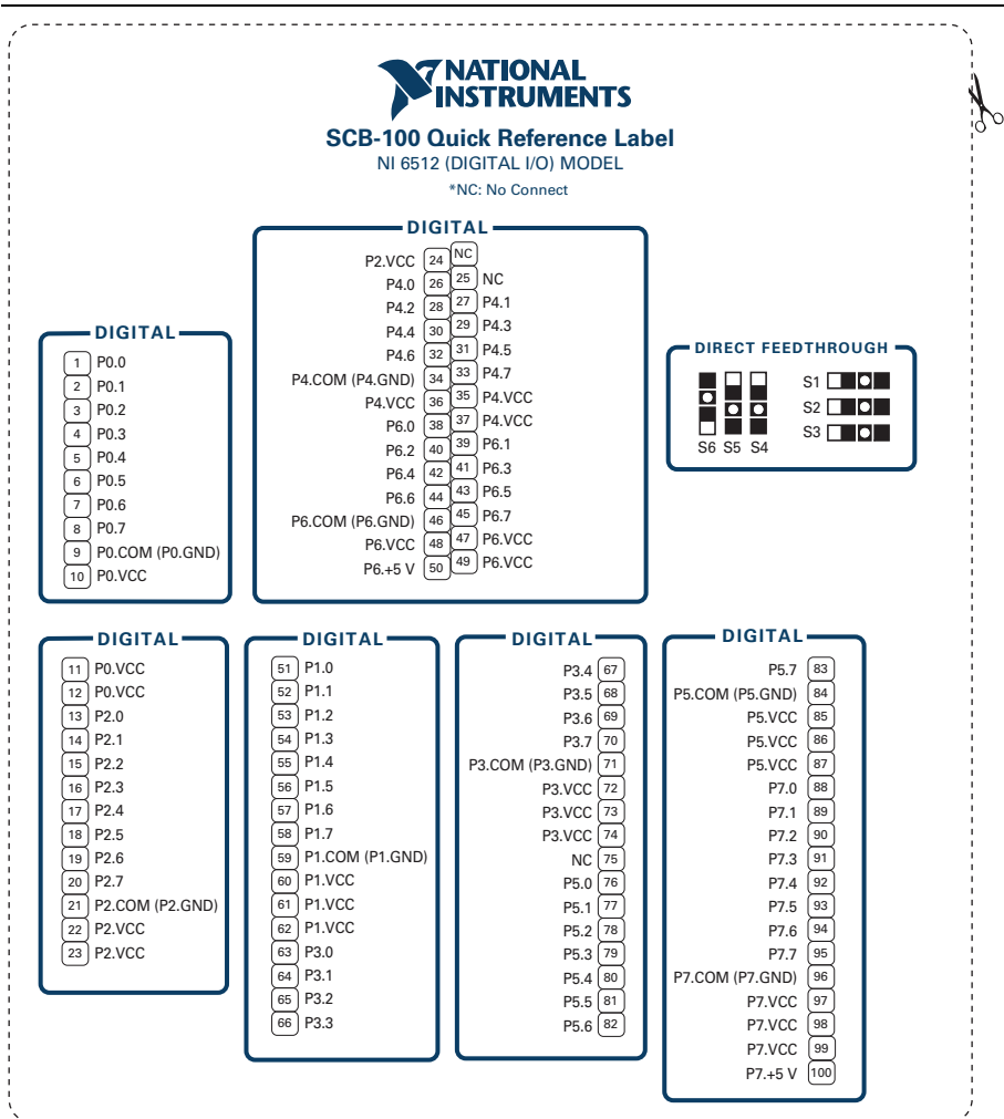
Figure 4. NI 6512
