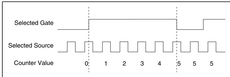
Figure 2-7. Single Pulse-Width Measurement
