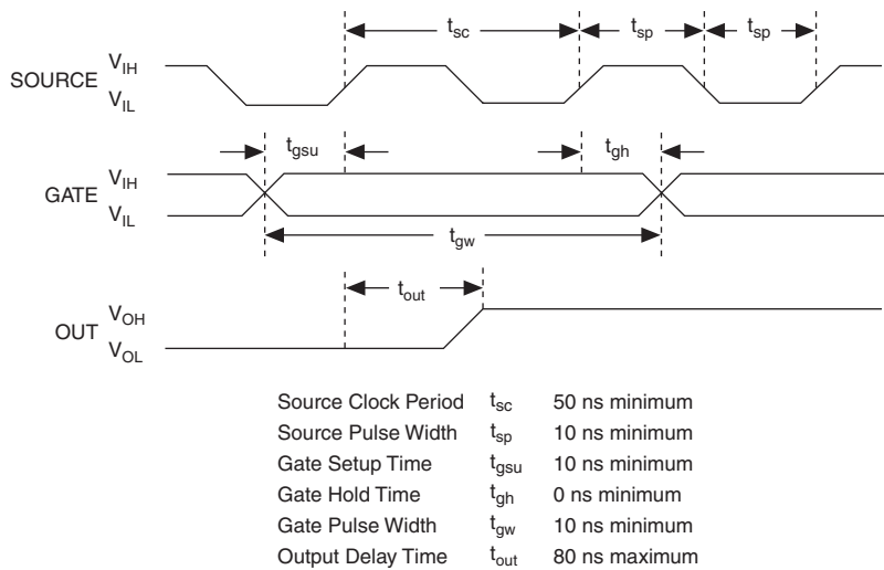
Figure 5-2. Gate and Source Input Timing Requirements
