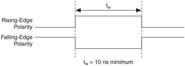
Figure 3-4. ao/StartTrigger Timing Requirements
