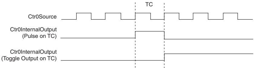
Figure 5-5. Ctr0InternalOutput Signal Behavior
