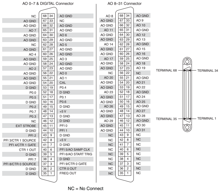
Figure 2-4. NI 6723 68-68-Pin Extended AO I/O Connector Pinout
