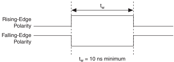
Figure 5-4. Ctr0Gate Timing Requirements
