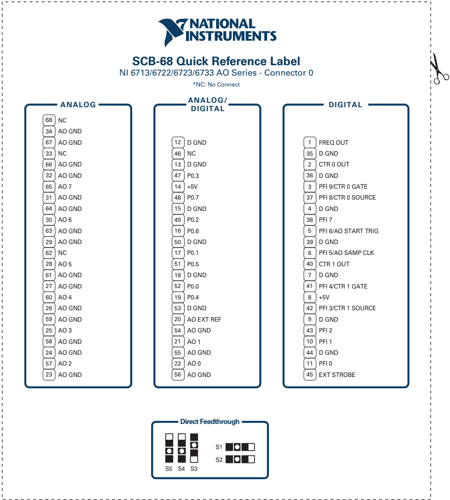
Figure 4. NI 6713/6722/6723/6733 Connector 0
