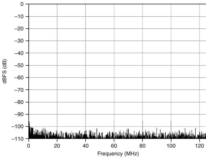
Figure 9. Terminated Input
