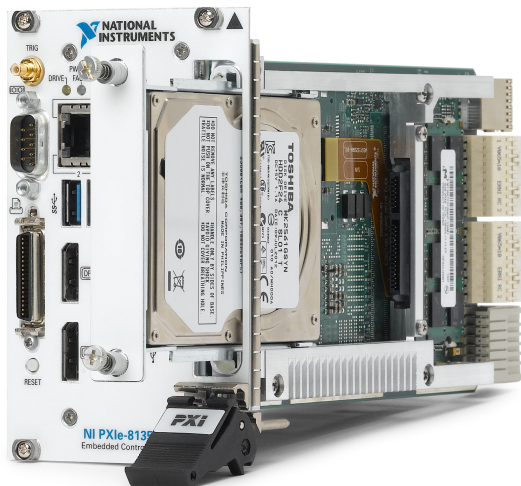
Figure 3: The PXIe-8135 offers a removeable hard disk drive.
