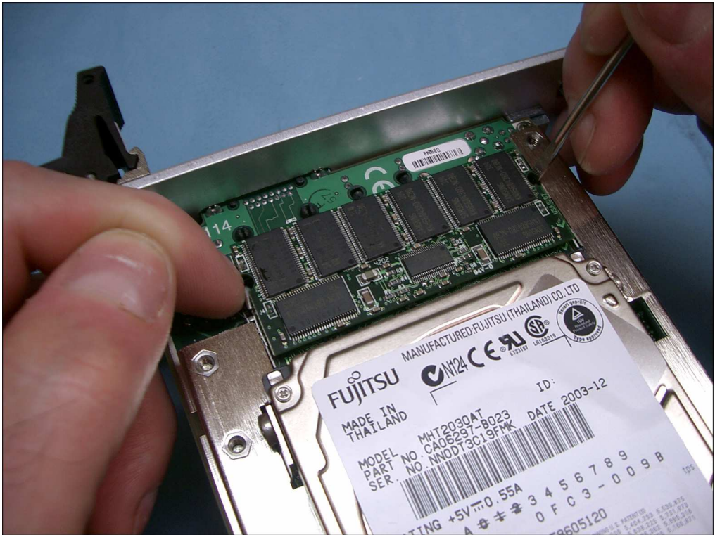
Figure 1. Removing the Memory Module
