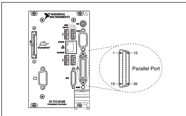
Figure 3-6. Parallel Port Connector Location and Pinout
