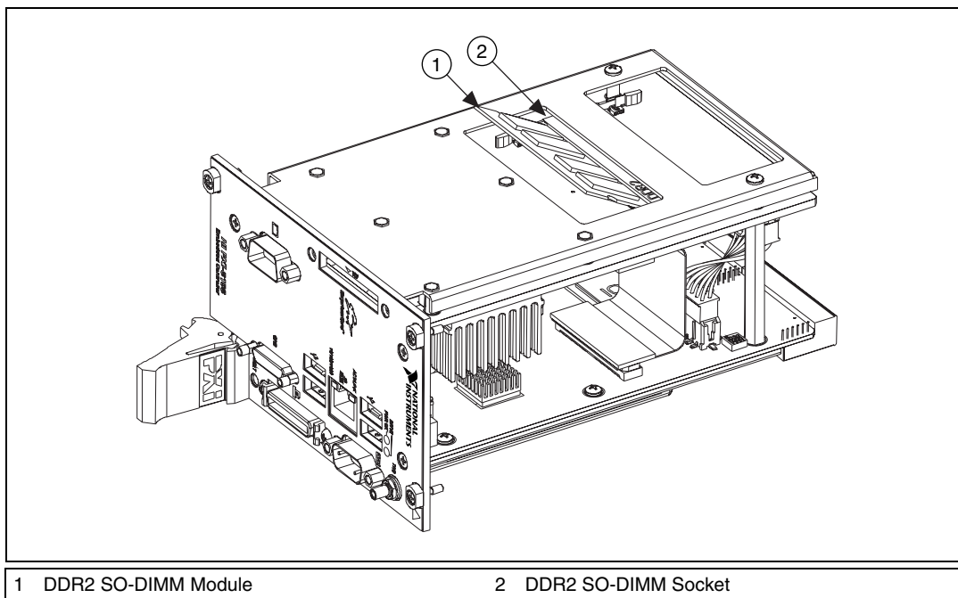
Figure 4-3. Installing a DDR2 SO-DIMM in an NI PXI-8195/8196 Controller
