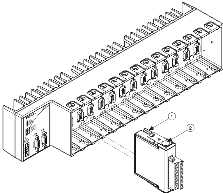
Figure 12. Installing an I/O Module in the Chassis
