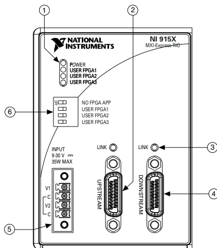
Figure 1. NI 9157/9159 Front Panel
