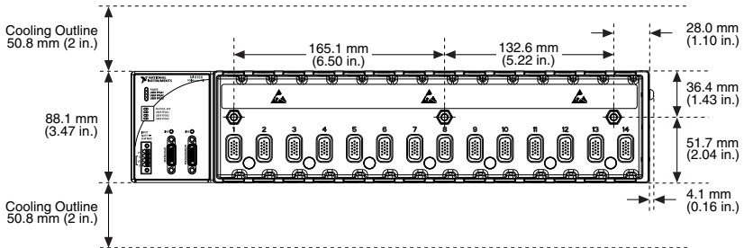
Figure 4. NI 9157/9159, Front View with Dimensions
