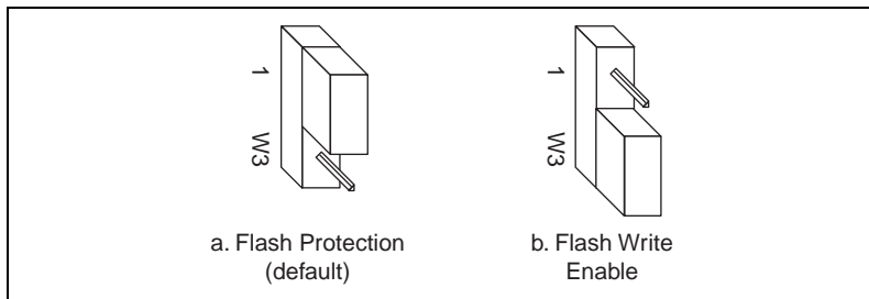
Figure 2. Flash Enable/Disable Jumper Settings
