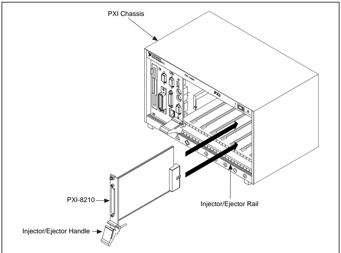
Figure 1. Installing the PXI-8210 into a PXI/CompactPCI Chassis
