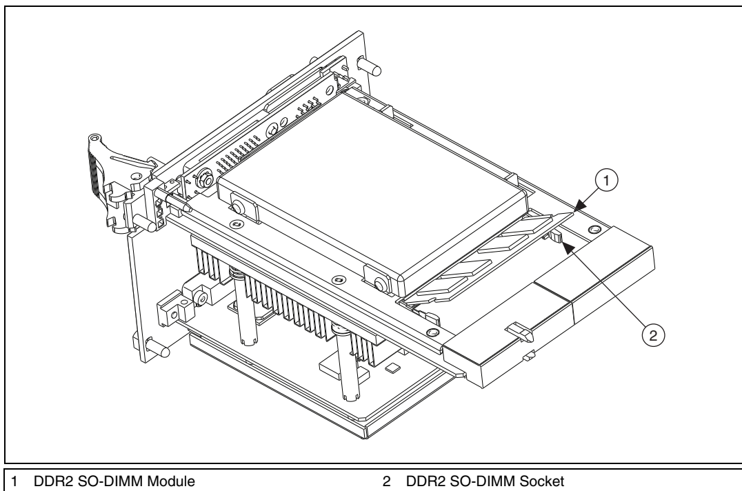
Figure 4-2. Installing a DDR2 SO-DIMM in an NI PXI-8110 Controller
