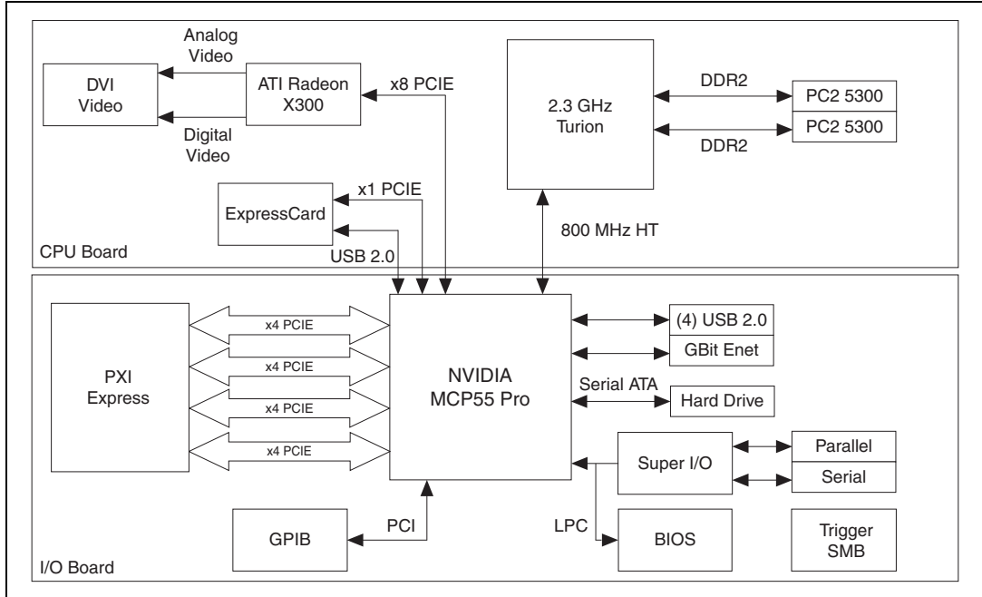
Figure 1-2. NI PXIe-8130 CPU Board and I/O Board
