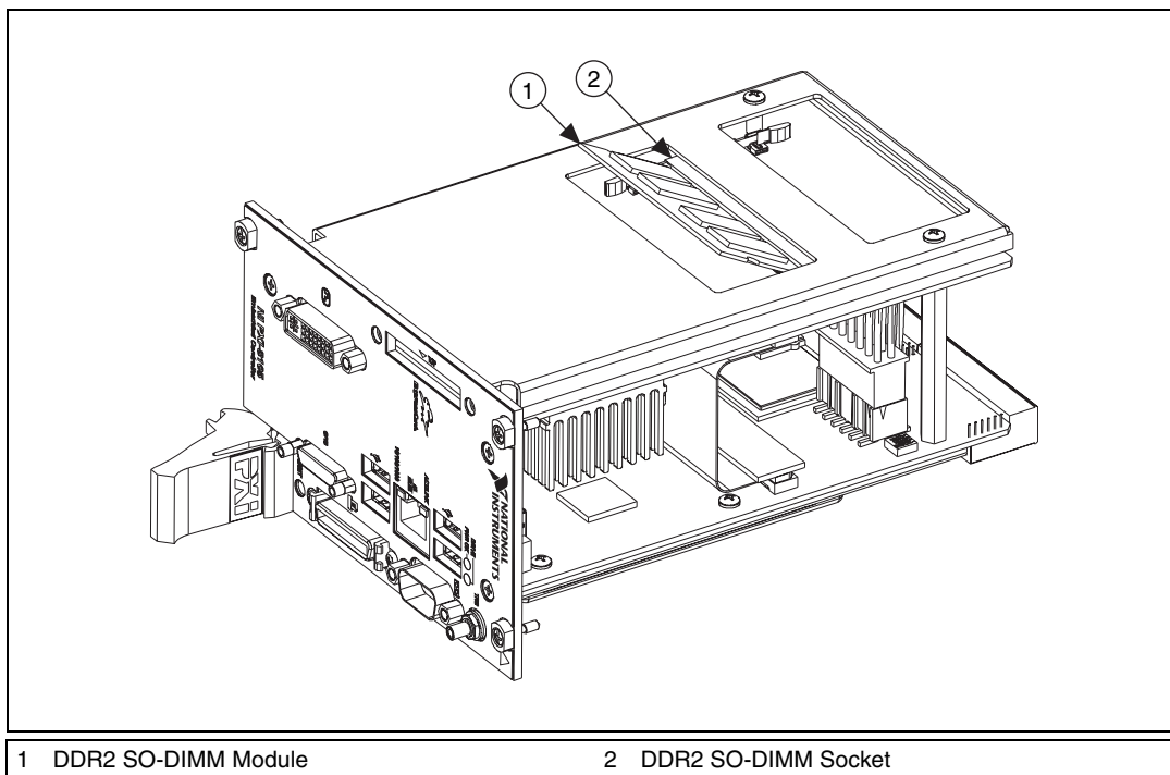
Figure 4-2. Installing a DDR2 SO-DIMM in an NI PXI-8105 Controller
