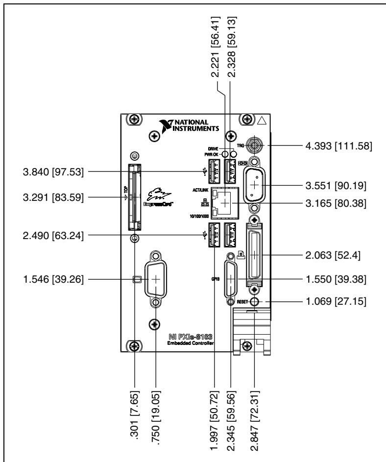
Figure 3-1. NI PXIe-8103 Front Panel Layout and Dimensions
