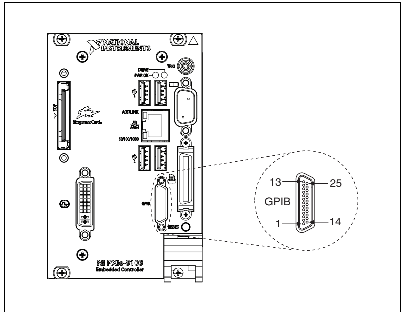
Figure 3-8. GPIO Connector Location and Pinout
