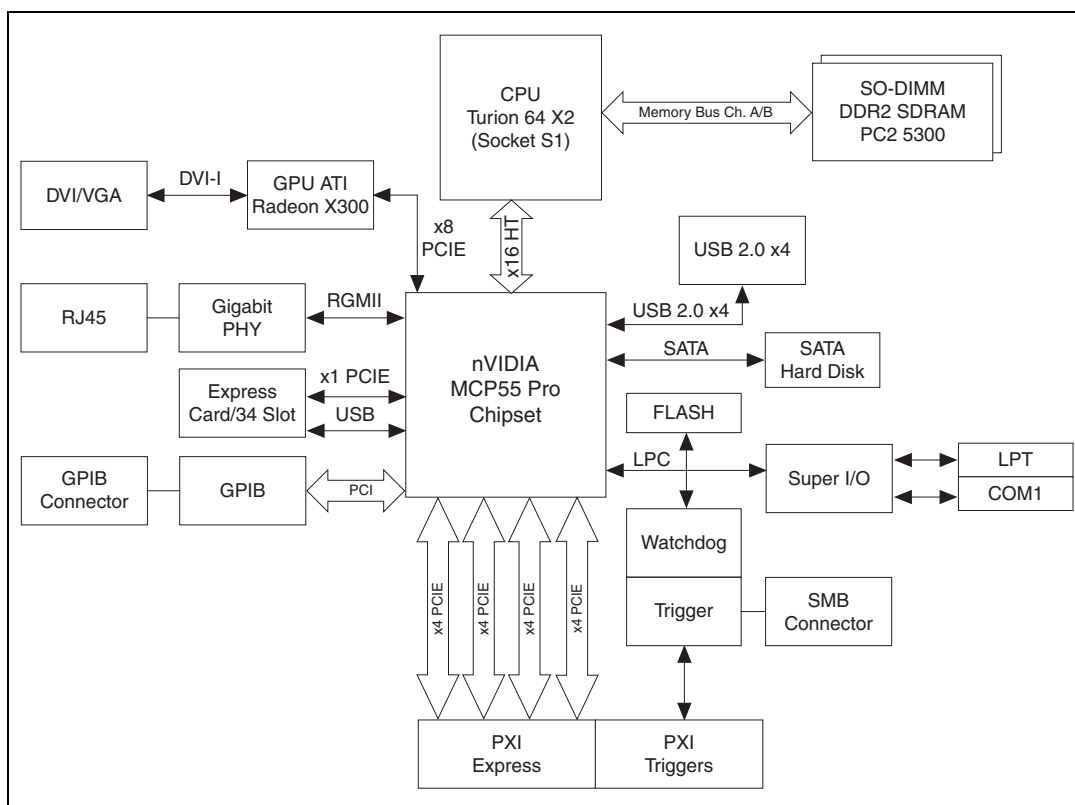
Figure 1-1. NI PXIe-8130 Block Diagram
