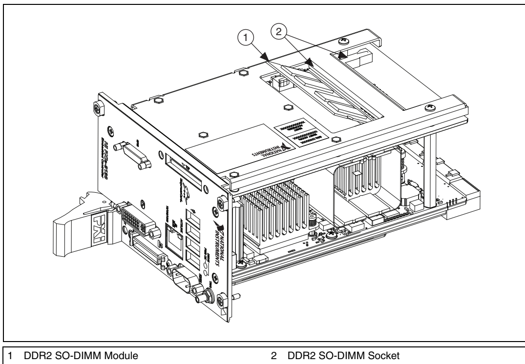
Figure 4-2. Installing a DDR2 SO-DIMM in an NI PXIe-8130 Controller
