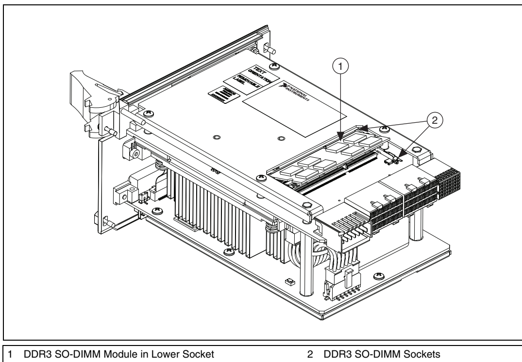
Figure 4-2. Installing a DDR3 SO-DIMM in an NI PXIe-8133 Controller
