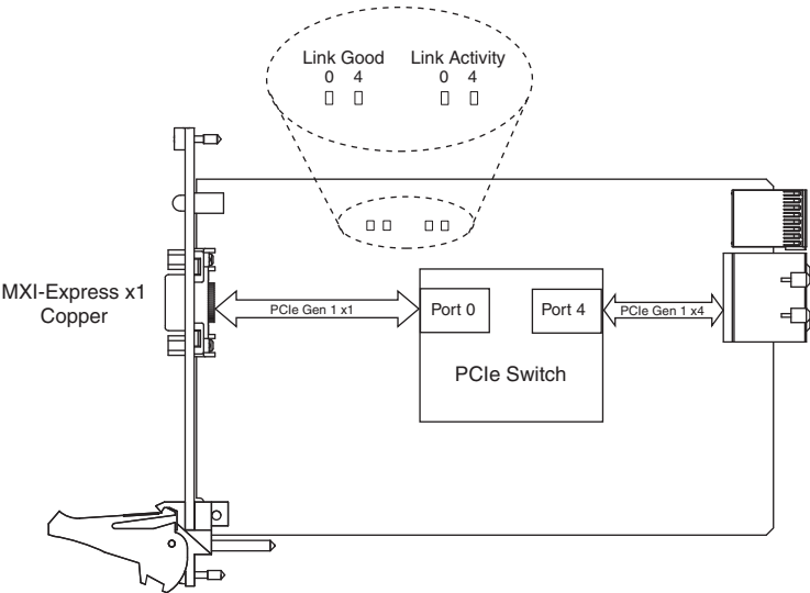
Figure 3-8. NI PXIe-8364 (193970x-01L) Onboard LED Locations
