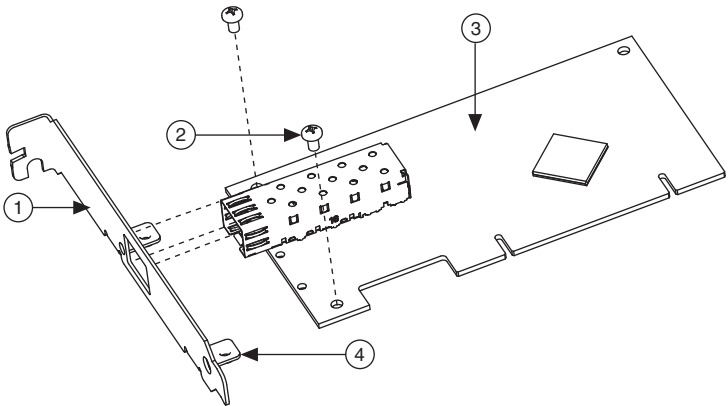
Figure 3-4. Removing Bracket
