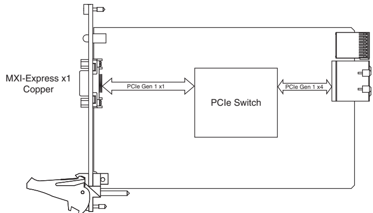
Figure 1-10. NI PXIe-8364 (193970x-01L) Block Diagram
