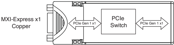
Figure 1-11. NI ExpressCard-8360 (198266x-01L) Block Diagram
