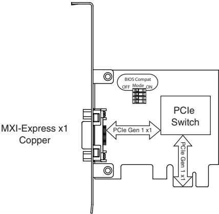
Figure 1-4. NI PCIe-8362 (190735x-01L) Block Diagram
