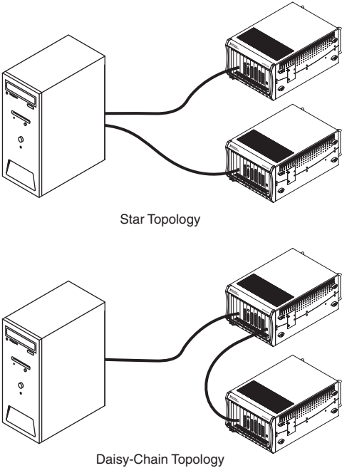
Figure 1-13. Example MXI-Express x1 System Expansion Topologies
