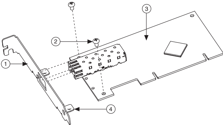
Figure 3-4. Removing Bracket
