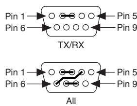
Figure 6. RS-232 Loopback
