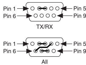
Figure 6. RS-232 Loopback
