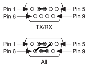
Figure 6. RS-232 Loopback
