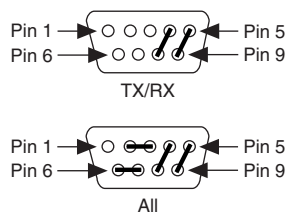
Figure 8. RS-485/422 Loopback
