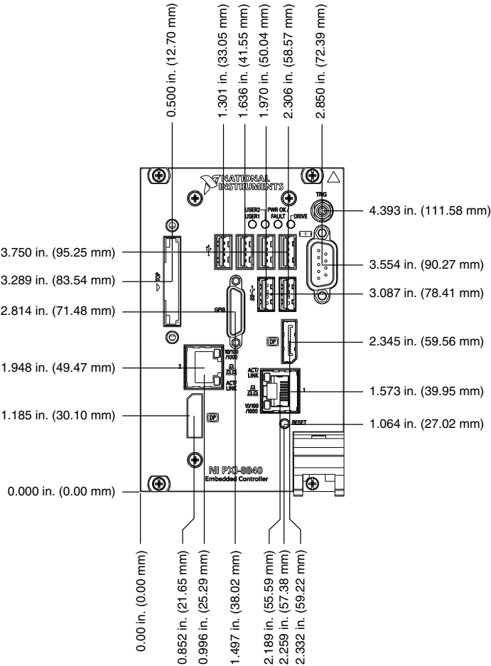
Figure 4. NI PXI-8840 Front Panel Layout and Dimensions
