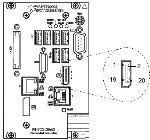
Figure 5. DisplayPort Connector Location and Pinout
