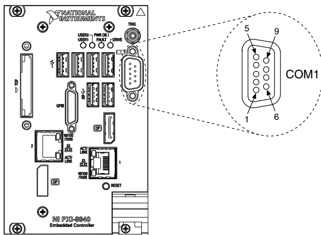
Figure 6. COM1 Connector Location and Pinout
