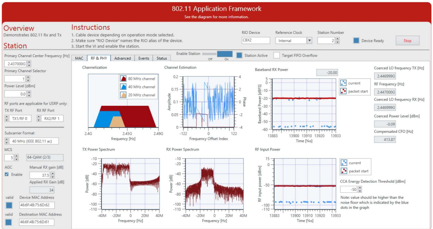
Figure 8 Application Framework RF & PHY Tab
