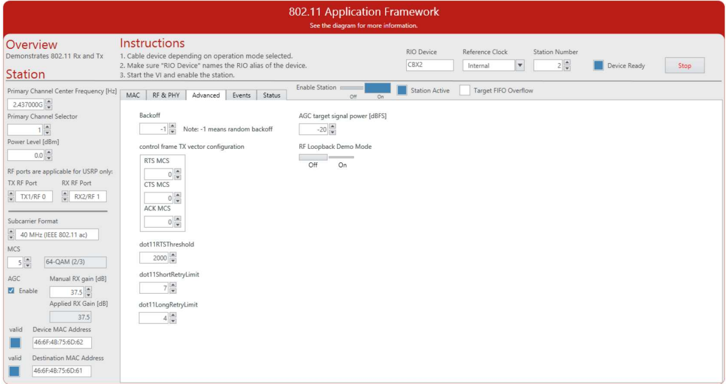
Figure 9 Application Framework Advanced Tab
