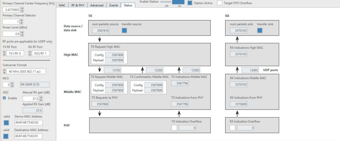
Figure 11 Application Framework Status Tab
