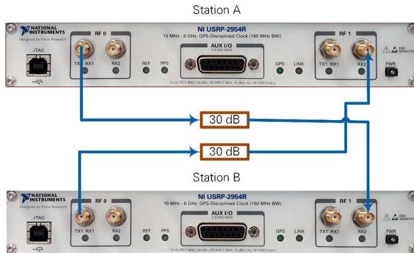
Figure 2 Cabled Connection of USRP RIO Devices
