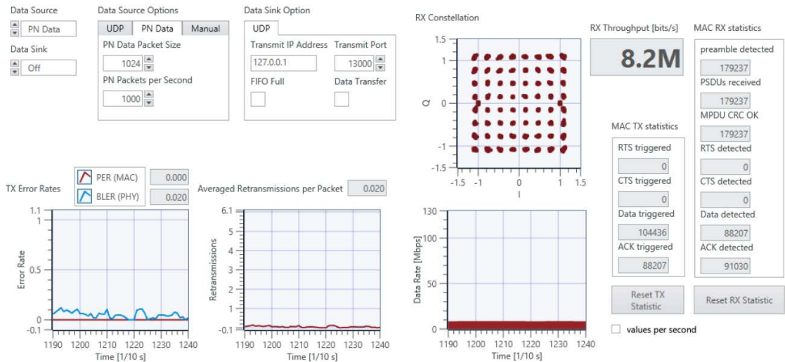
Figure 6 Application Framework User Interface – Station A: MAC Tab
