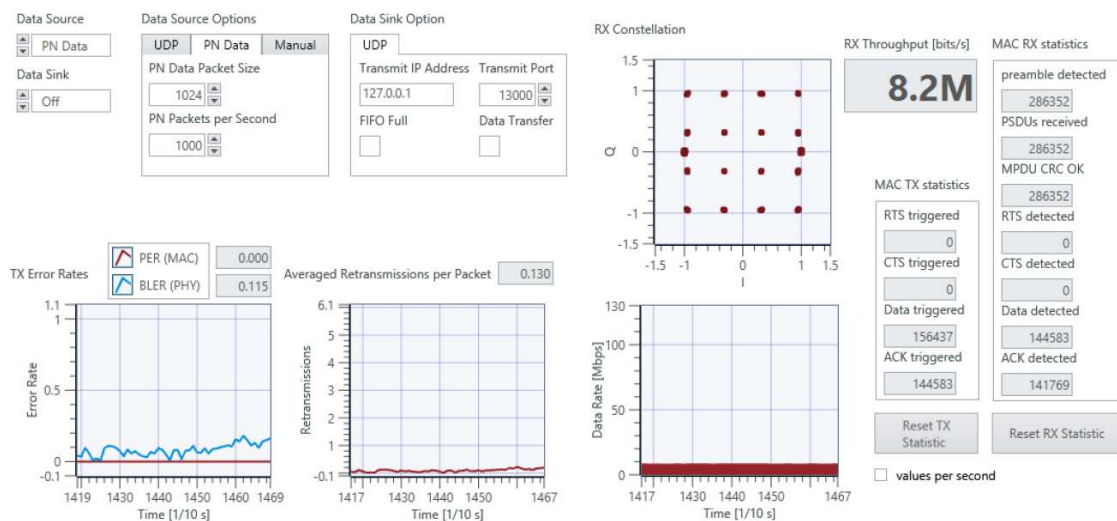
Figure 7 Application Framework User Interface – Station B: MAC Tab
