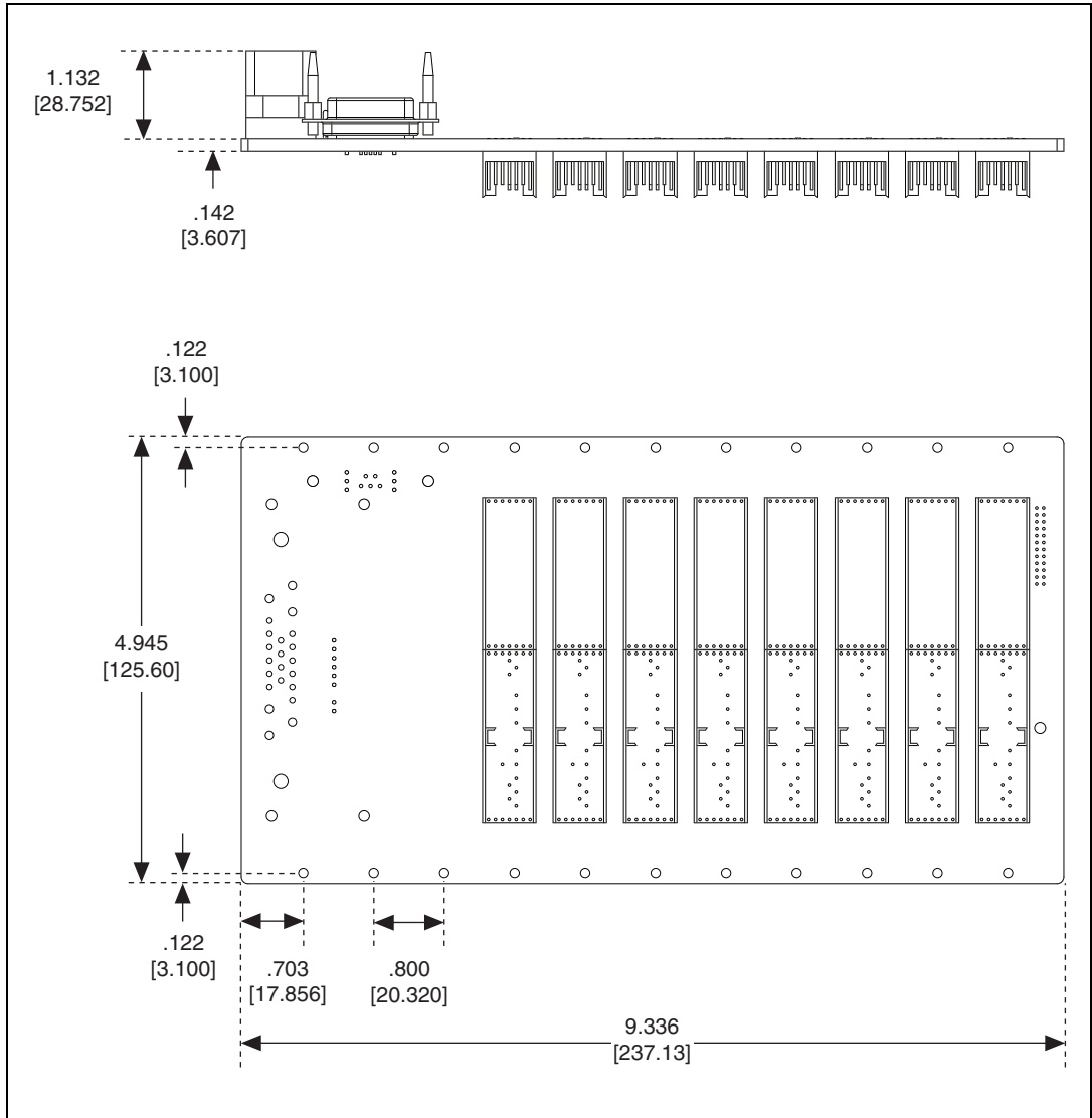
Figure 2. Dimensions
