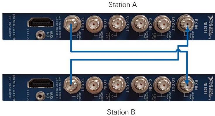
Figure 3 FlexRIO Adapter Module Cabled Connection
