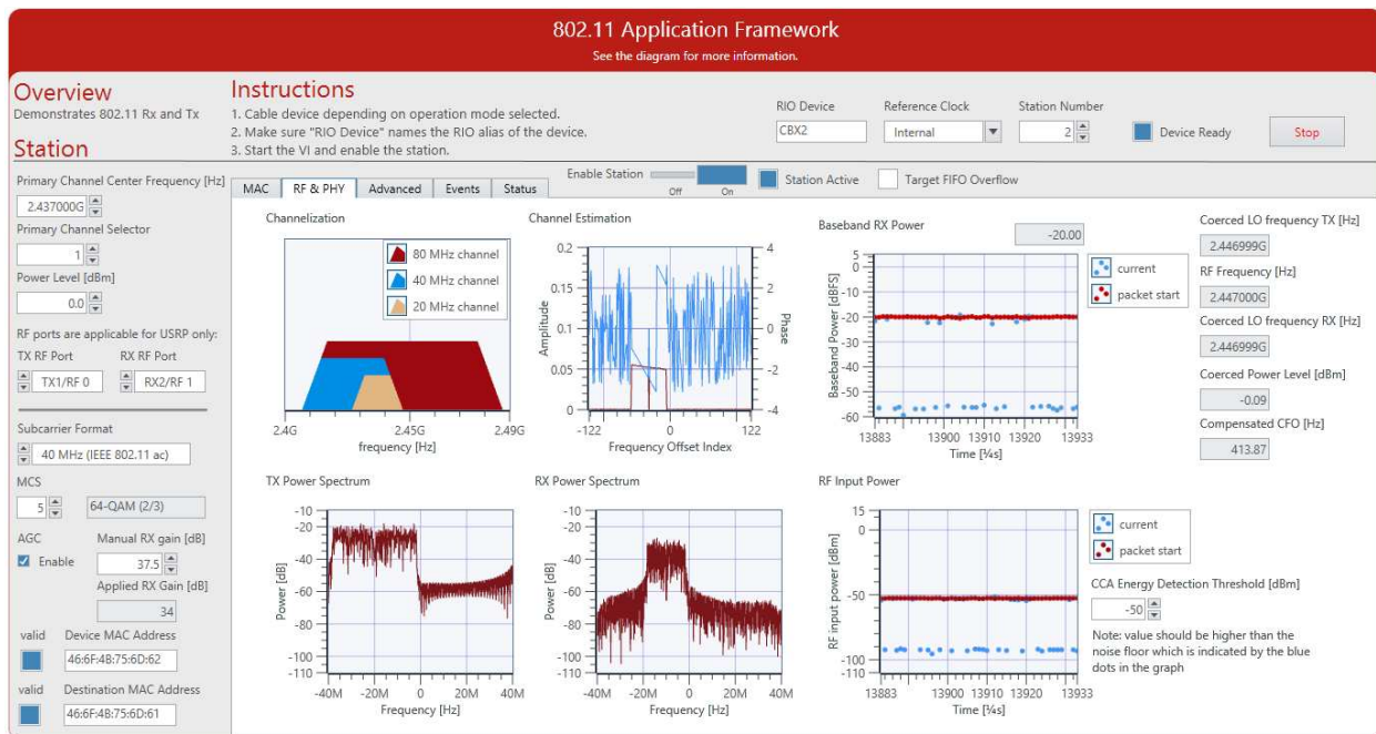
Figure 8 Application Framework RF & PHY Tab
