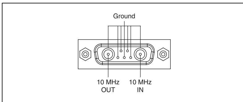
Figure 5. J40 Connector
