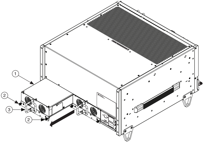
Figure 3-1. Removing Power Supply from PXIe-1086 Chassis
